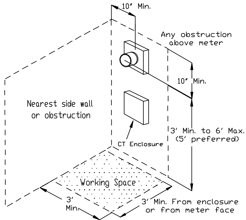
Meter socket minimum clearances.
