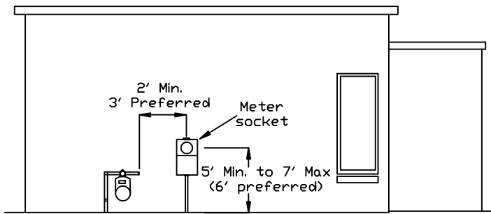
Meter socket height and gas meter clearance.
