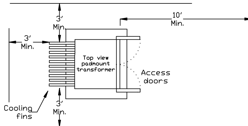
Clear working space for padmount equipment.
