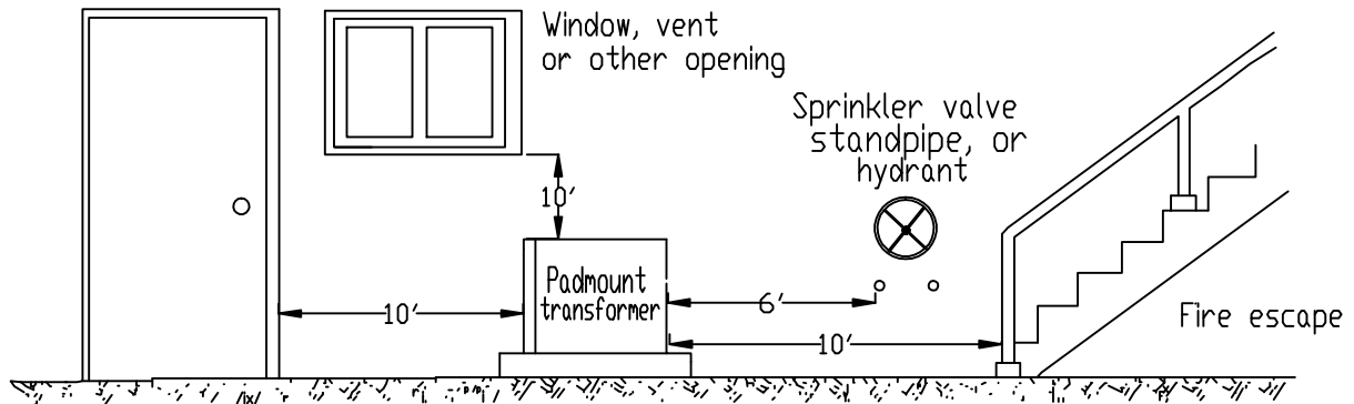
Clearances for padmount transformer.
